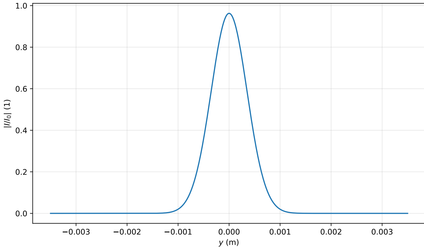
Intensity profile I(x=0, y, z=0.478)/I_0 , P_{in}=0.1P_{cr} , artificial time
